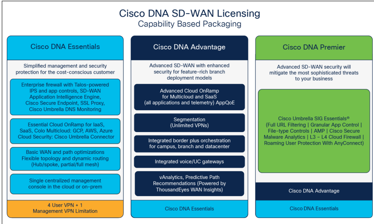
Figure 3. Cisco DNA Software subscription licensing for SD-WAN and routing
